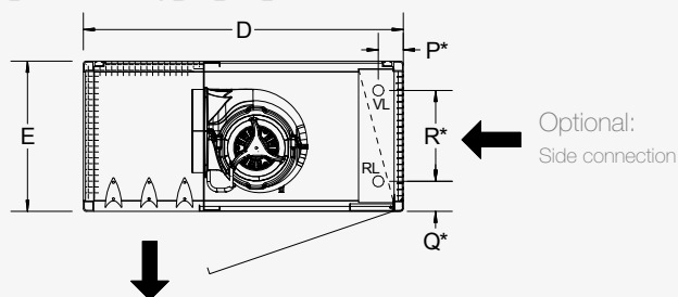
SIDE VIEW/SECTION
